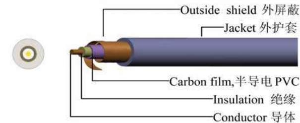
DX0281A Difibrillation cable 除颤器手柄线
